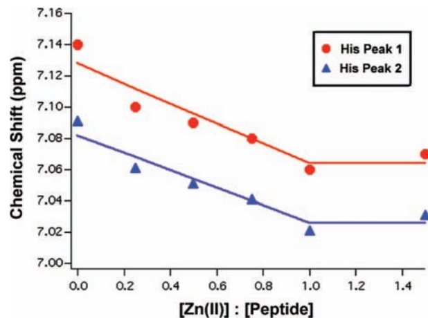
Figure 4. Chemical shift vs [Zn(II)] for the two Mst-HH C4 histidine proton resonances (1 mM Mst-HH, 10 mM Tris pH = 6.0, 150 mM NaCl).
