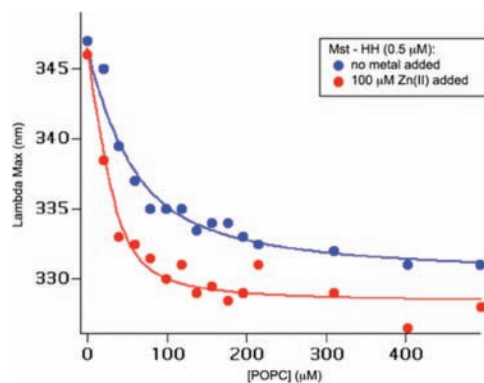
Figure 9. Mst-HH wavelength of maximum tryptophan emission vs [POPC]. Results from fitting the data to a simple dissociation equilibrium (eq 3) with a lipid site size of 80 are depicted as curves through the data points.
